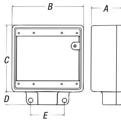
Fig. B Dead-End
