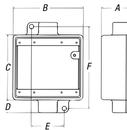
Fig. C Thru-Feed
